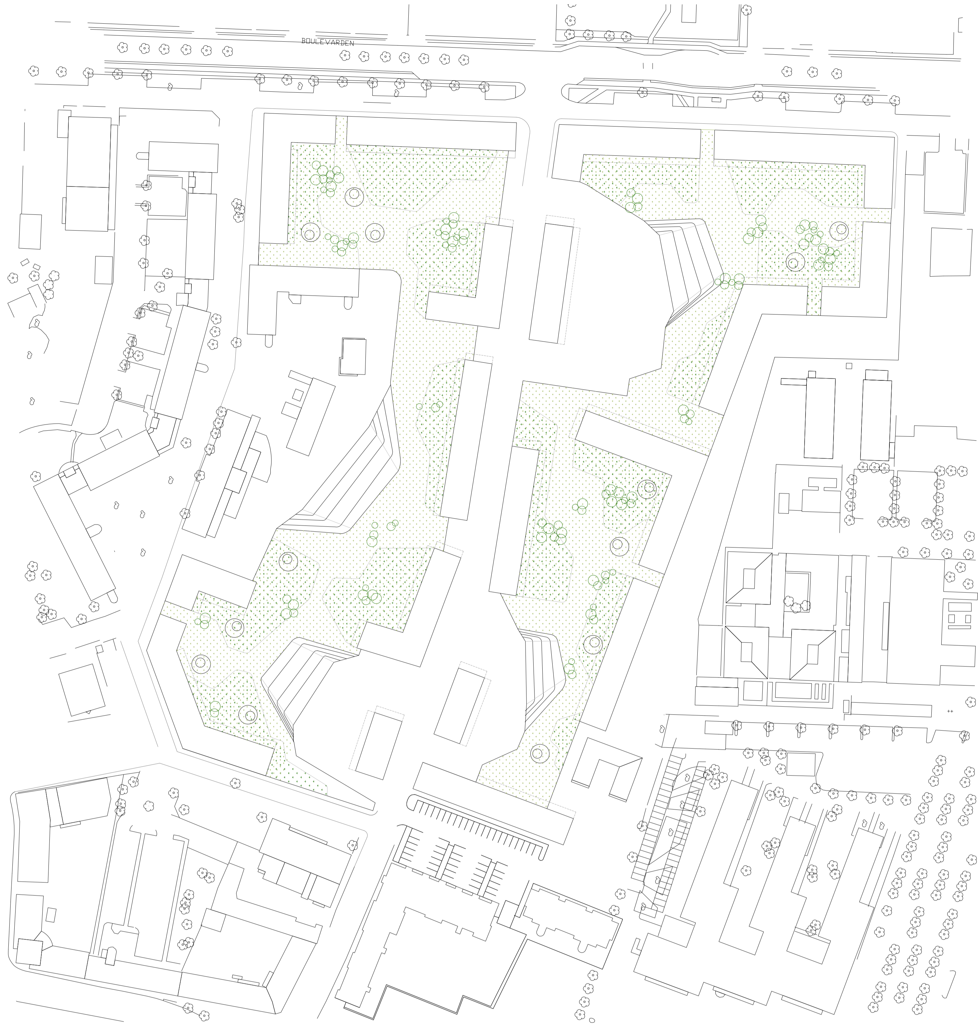
LEVEL +4 M
